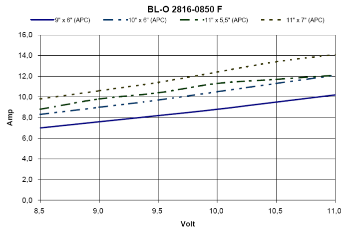
BL-O 2816-0850F - current / voltage with different propellers
