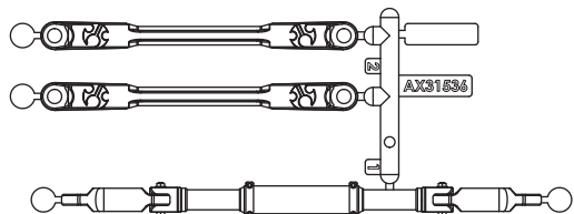
AX31536 (x1) SCX10 II Steering link SCX10 II-Lenkstange Tringlerie de direction SCX10 II Collegamento sterzo SCX10 II
