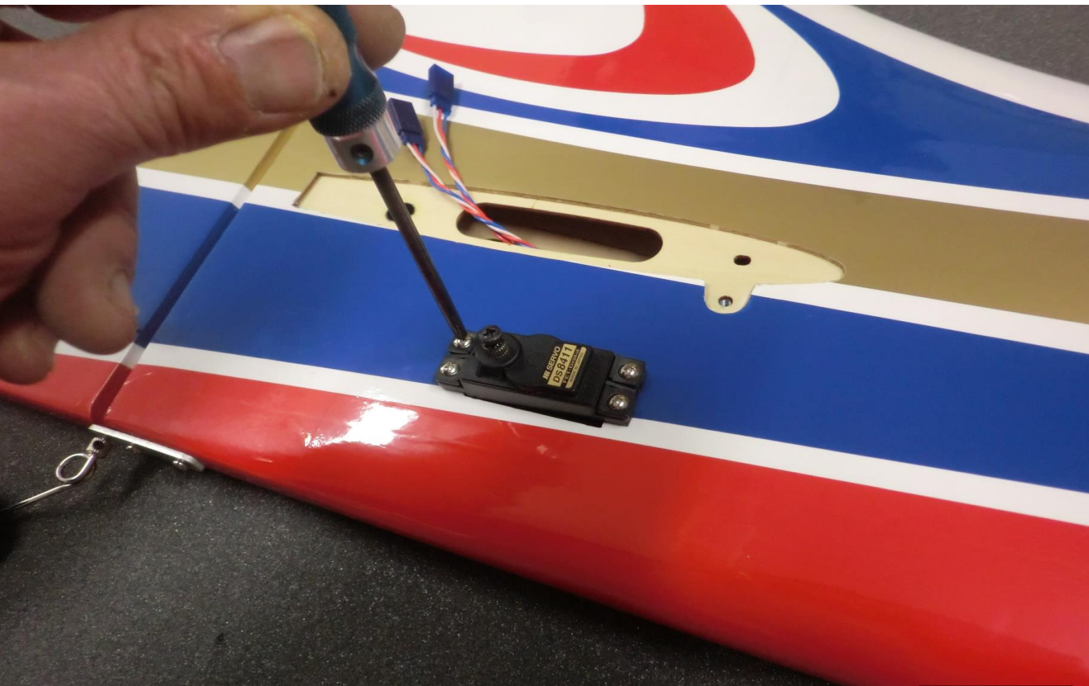
Rudder installation
