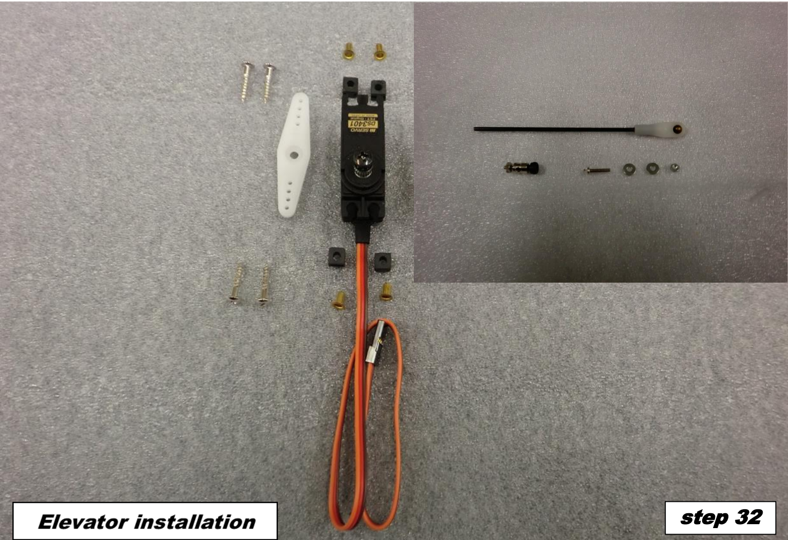
Elevator installation
