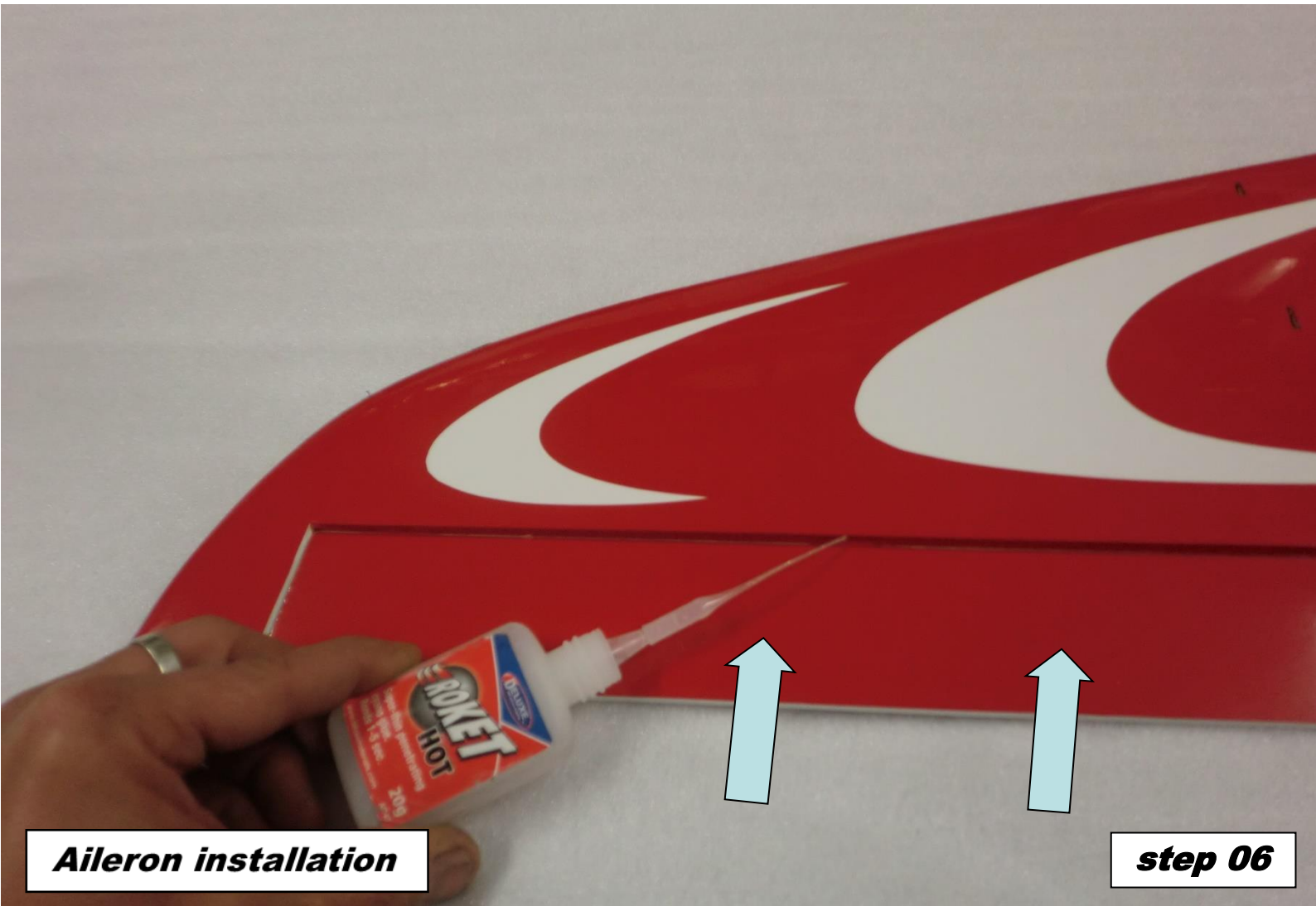
Aileron installation
