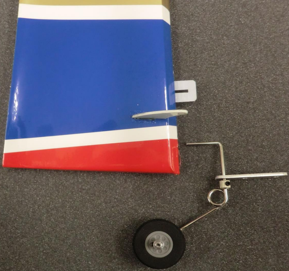
Rudder installation
