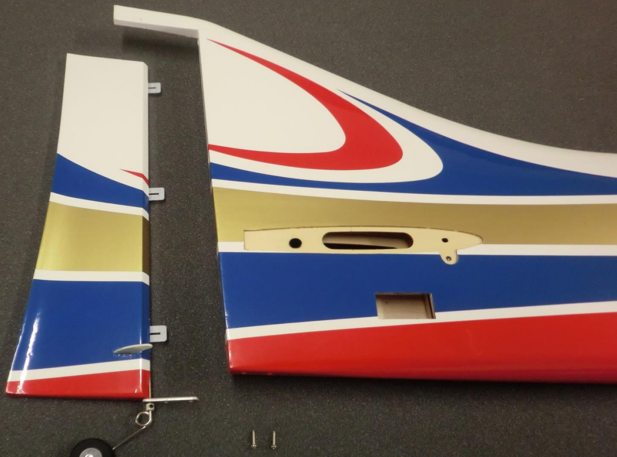
Rudder installation
