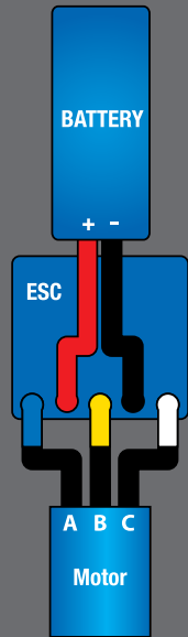
ESC/Motor Wiring Diagram
