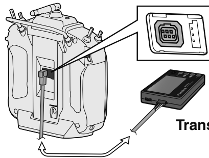
Trainer jack of the transmitter.
